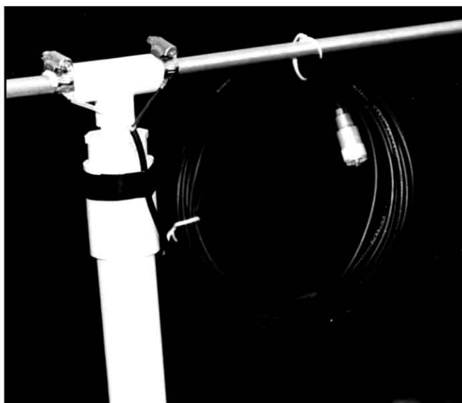
Figure 3—Tape the coax to the mast below the T to keep the connections from flexing in the wind. The remaining coax is shown rolled up and attached to the antenna in preparation for portable operation.
